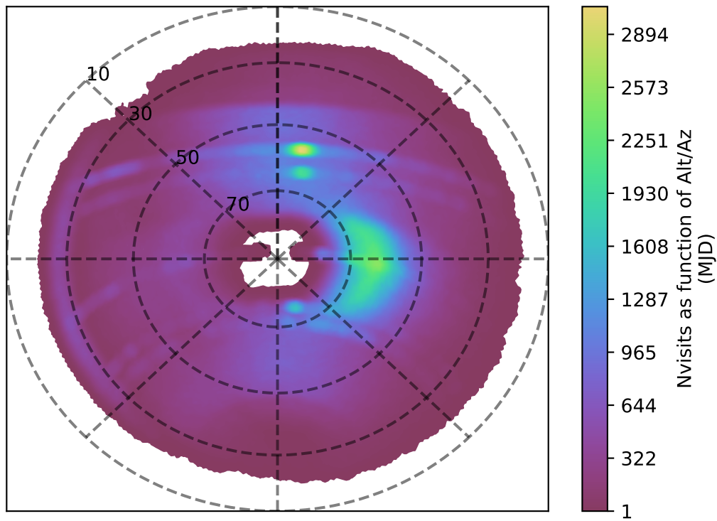
ddf_acor_sf25_lsf30_lsr50_v3.4_10yrs r band: Nvisits as function of Alt/Az
