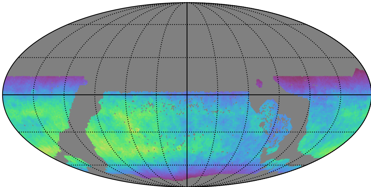
ddf_acor_sf25_lsf30_lsr50_v3.4_10yrs WFD y band: Normalized Teff
