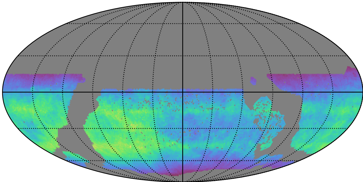
ddf_acor_sf25_lsf30_lsr50_v3.4_10yrs WFD i band: Normalized Teff
