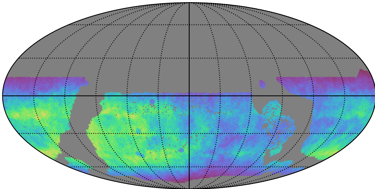
ddf_acor_sf25_lsf30_lsr50_v3.4_10yrs WFD g band: Normalized Teff
