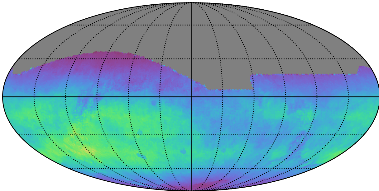
ddf_acor_sf25_lsf30_lsr50_v3.4_10yrs All sky r band: Normalized Teff
