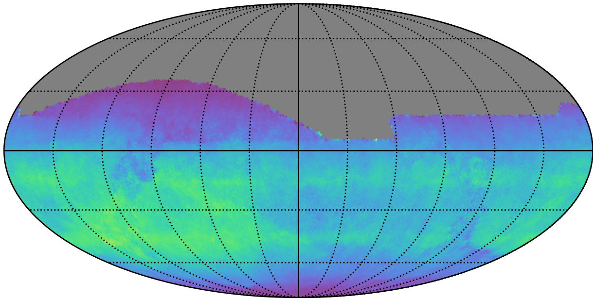
ddf_acor_sf25_lsf30_lsr50_v3.4_10yrs All sky i band: Normalized Teff
