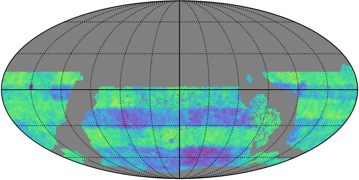
ddf_acor_sf25_lsf30_lsr50_v3.4_10yrs WFD: Normalized Proper Motion Uncert @ 24.0
