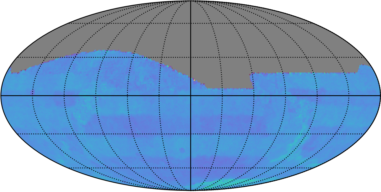
ddf_acor_sf25_lsf30_lsr50_v3.4_10yrs All sky: Normalized Proper Motion Uncert @ 24.0
