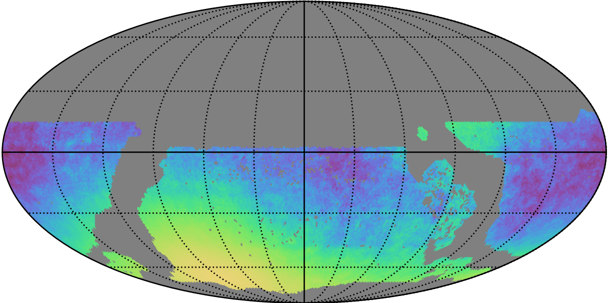
ddf_acor_sf25_lsf30_lsr50_v3.4_10yrs WFD y band only: Normalized Parallax Uncert @ 21.3
