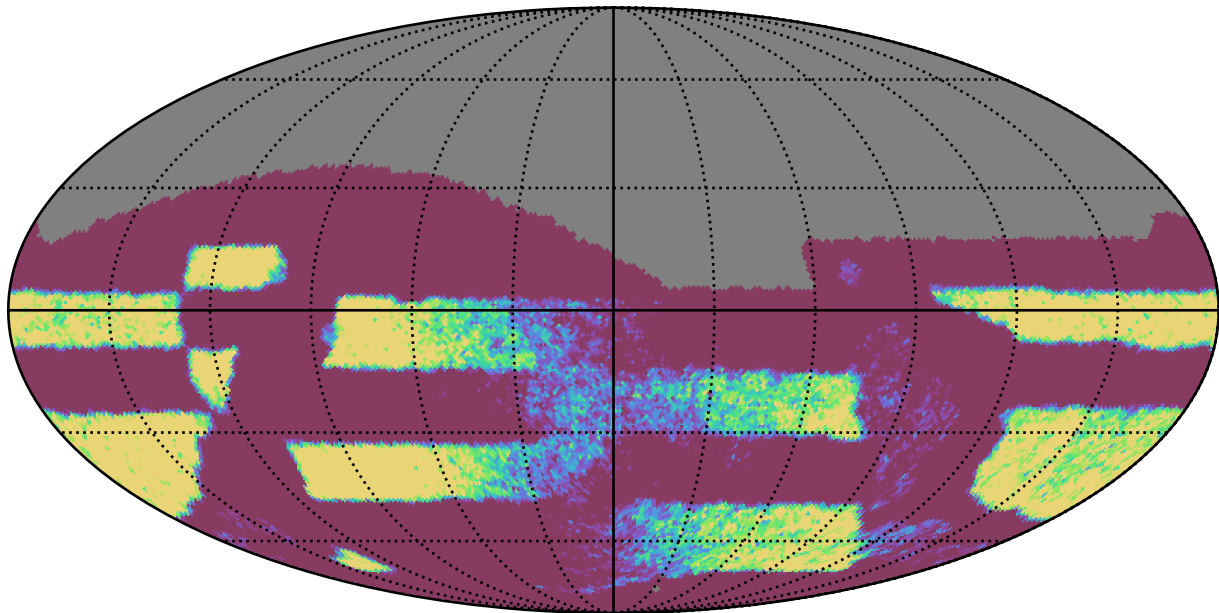
ddf_acor_sf25_lsf30_lsr50_v3.4_10yrs Yr 3-4 all bands: NVisits
