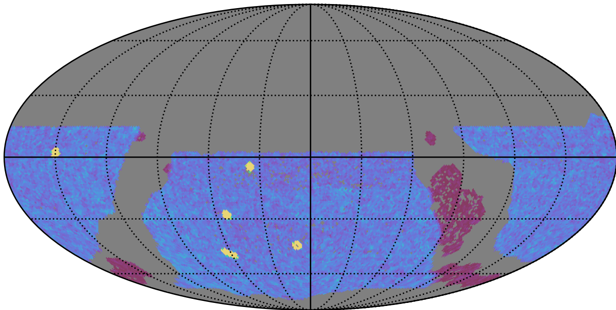
ddf_acor_sf25_lsf30_lsr50_v3.4_10yrs WFD y band: NVisits
