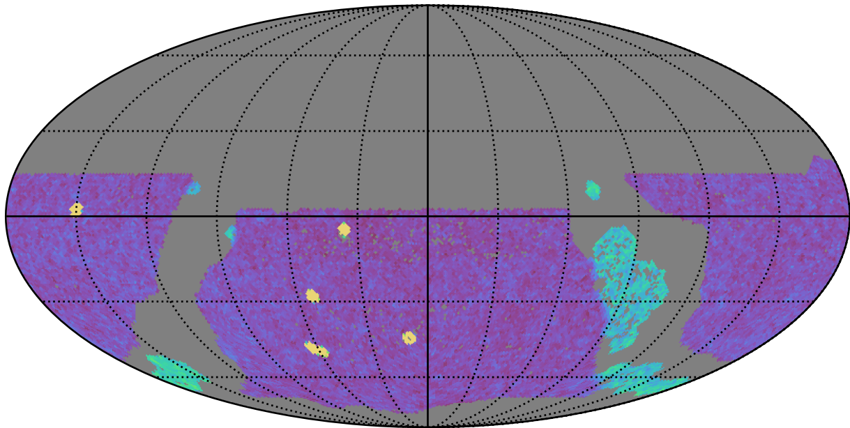
ddf_acor_sf25_lsf30_lsr50_v3.4_10yrs WFD g band: NVisits
