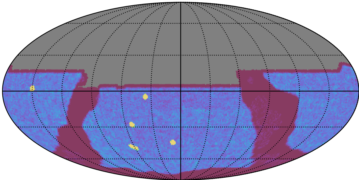
ddf_acor_sf25_lsf30_lsr50_v3.4_10yrs All sky y band: NVisits
