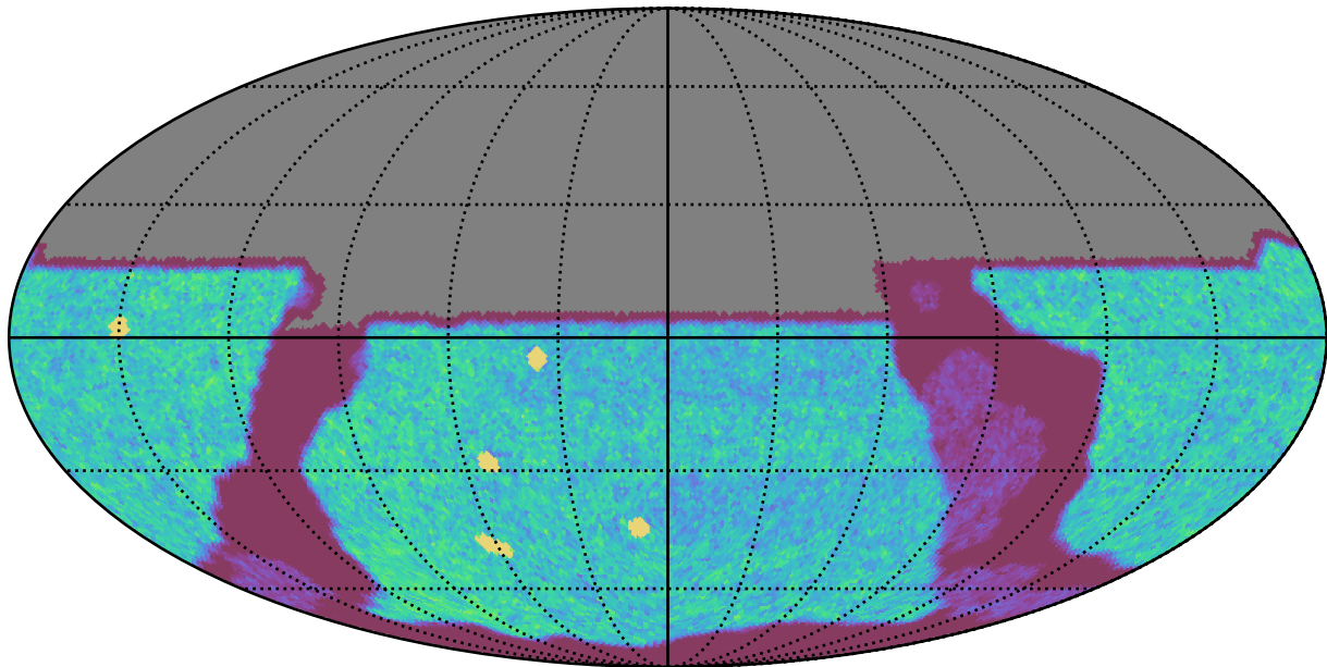
ddf_acor_sf25_lsf30_lsr50_v3.4_10yrs All sky u band: NVisits
