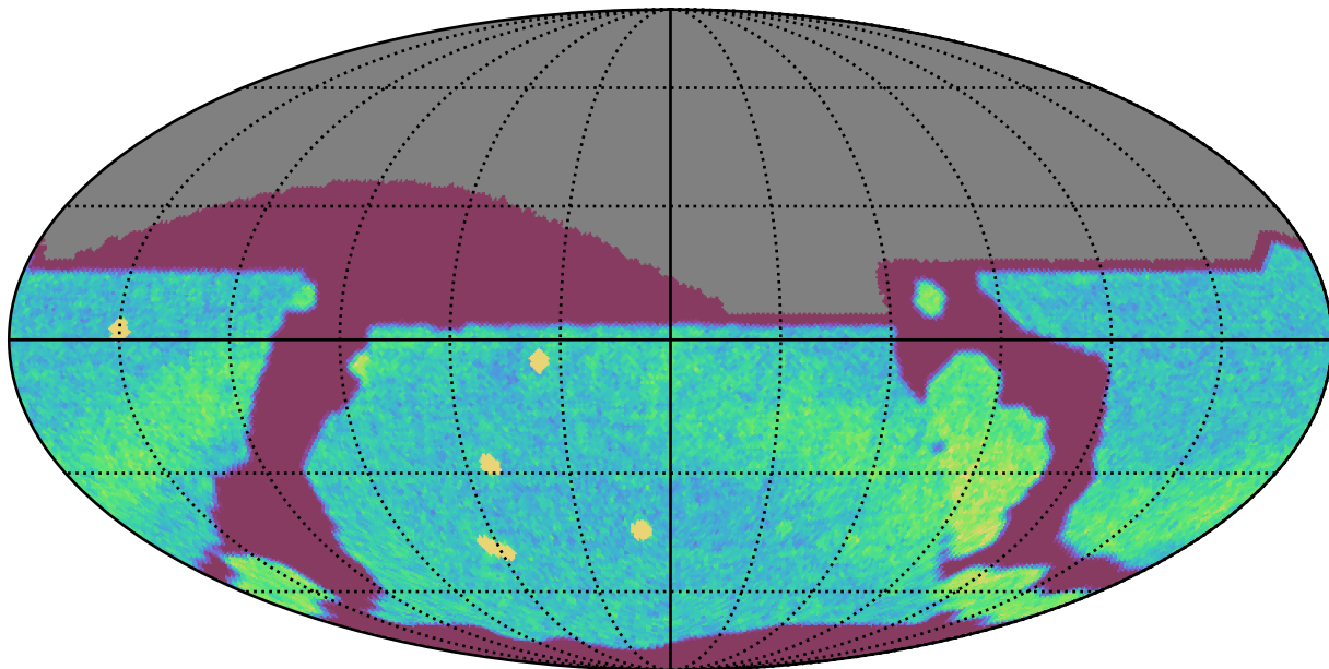
ddf_acor_sf25_lsf30_lsr50_v3.4_10yrs All sky r band: NVisits
