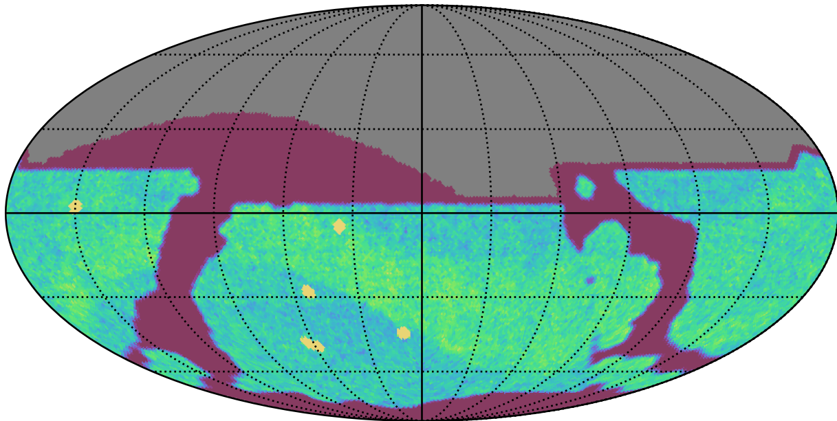
ddf_acor_sf25_lsf30_lsr50_v3.4_10yrs All sky i band: NVisits
