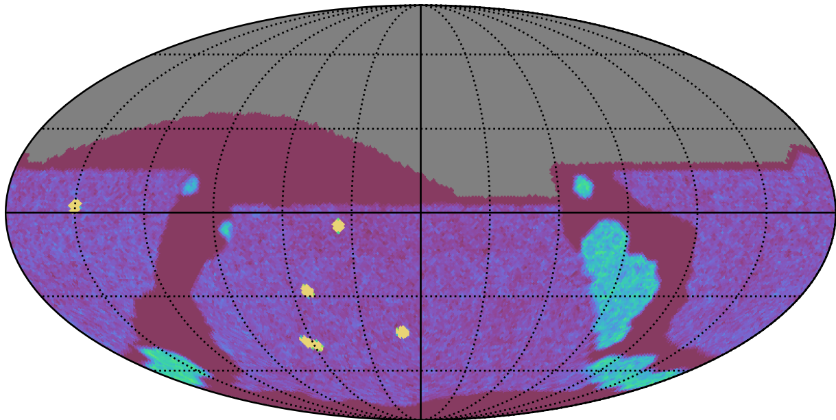
ddf_acor_sf25_lsf30_lsr50_v3.4_10yrs All sky g band: NVisits
