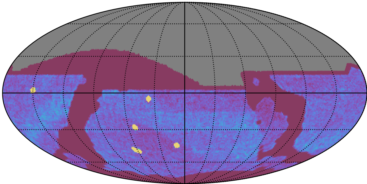
ddf_acor_sf25_lsf30_lsr50_v3.4_10yrs All sky all bands: NVisits
