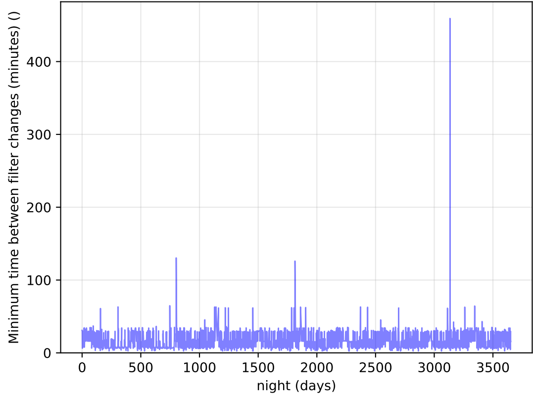
ddf_acor_sf25_Isf30_Isr50_v3.4_10yrs Per Night: Minimum time between filter changes (minutes)
