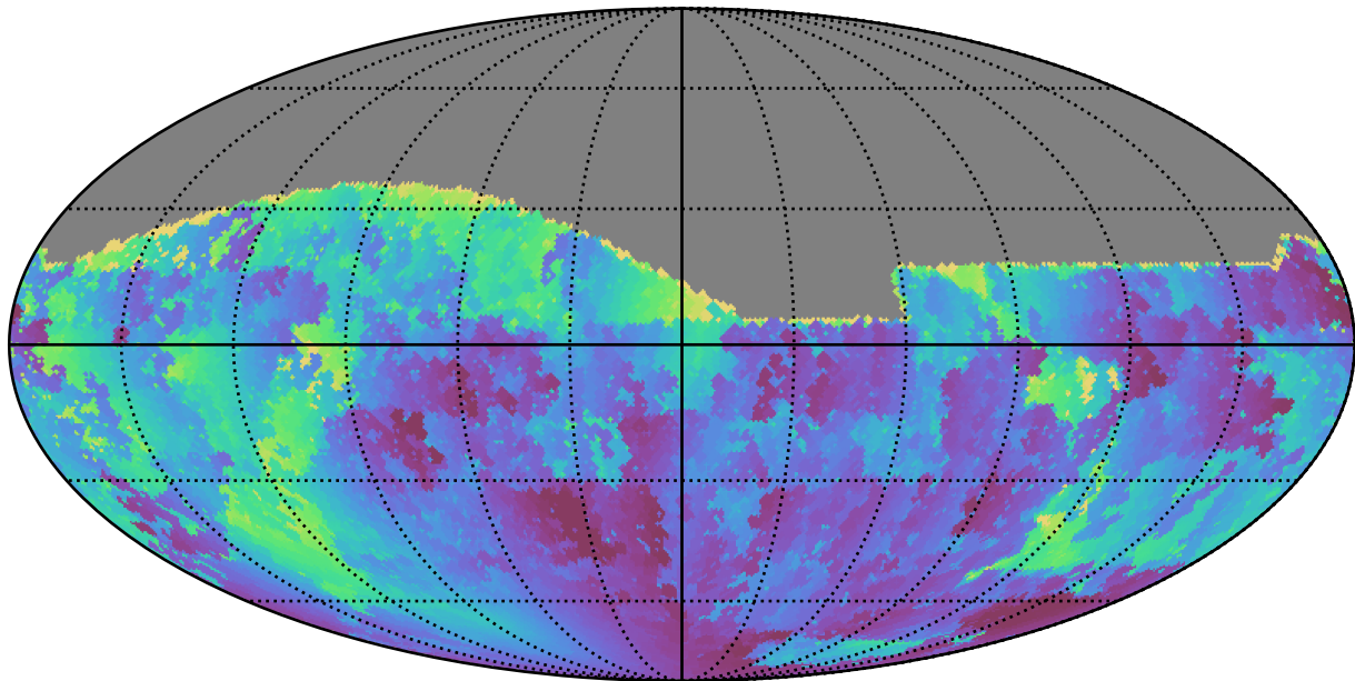
ddf_acor_sf25_lsf30_lsr50_v3.4_10yrs All sky g band: Min solarElong
