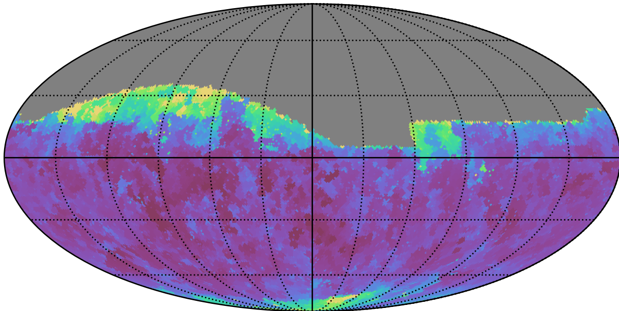
ddf_acor_sf25_lsf30_lsr50_v3.4_10yrs Yr 1 r band: Min seeingEff
