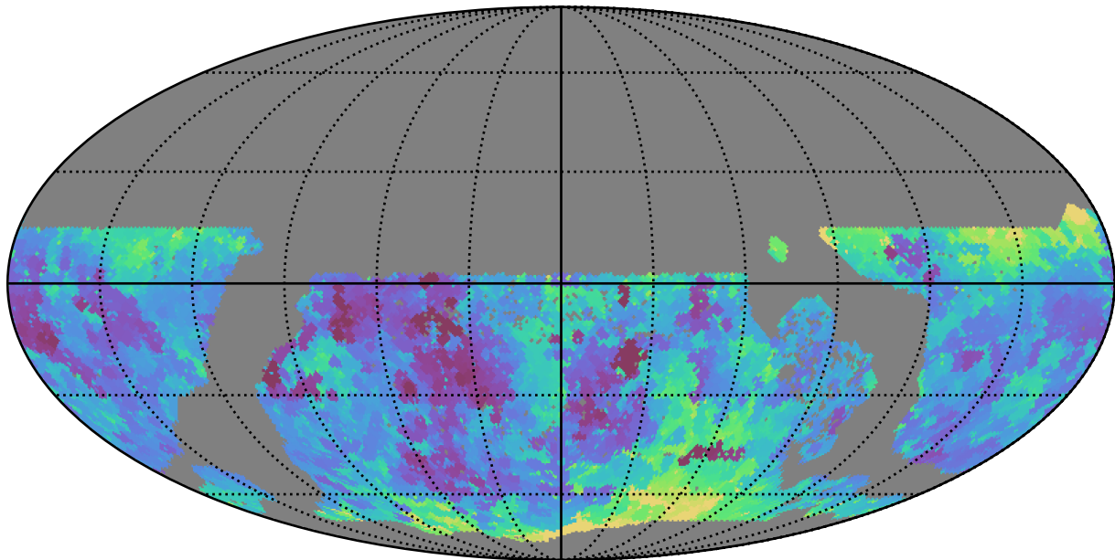
ddf_acor_sf25_lsf30_lsr50_v3.4_10yrs WFD g band: Min seeingEff
