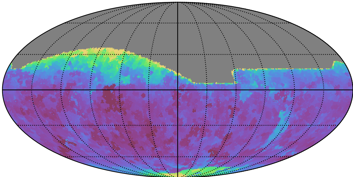
ddf_acor_sf25_lsf30_lsr50_v3.4_10yrs All sky z band: Min seeingEff
