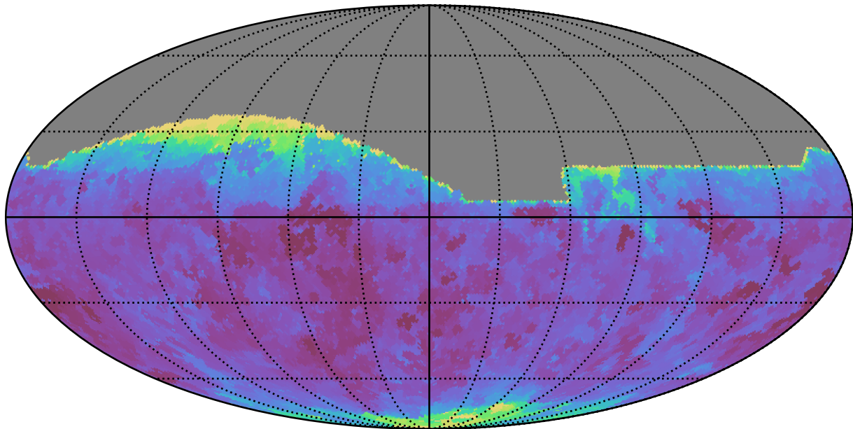
ddf_acor_sf25_lsf30_lsr50_v3.4_10yrs All sky r band: Min seeingEff
