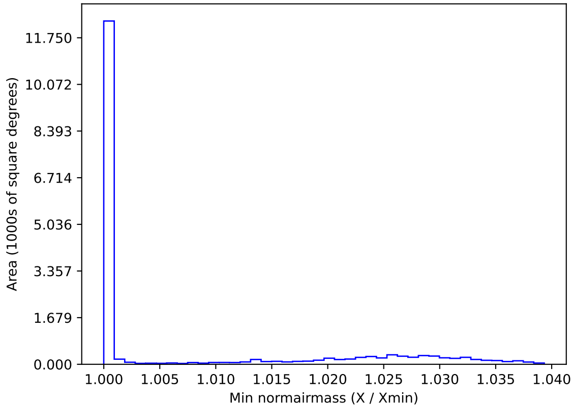
ddf_acor_sf25_lsf30_lsr50_v3.4_10yrs WFD y band: Min normairmass
