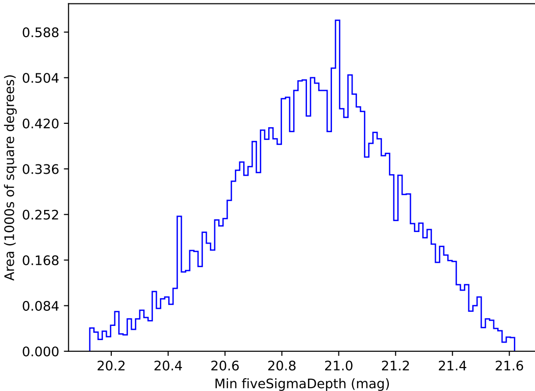
ddf_acor_sf25_lsf30_lsr50_v3.4_10yrs All sky y band: Min fiveSigmaDepth
