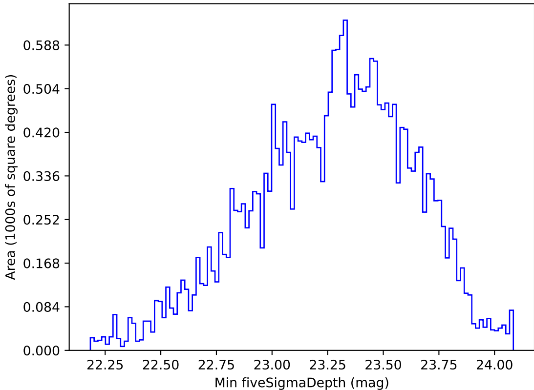
ddf_acor_sf25_lsf30_lsr50_v3.4_10yrs All sky g band: Min fiveSigmaDepth
