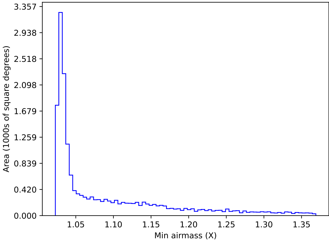
ddf_acor_sf25_lsf30_lsr50_v3.4_10yrs WFD y band: Min airmass
