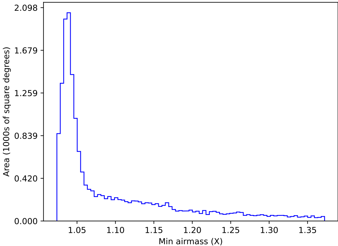
ddf_acor_sf25_lsf30_lsr50_v3.4_10yrs WFD u band: Min airmass
