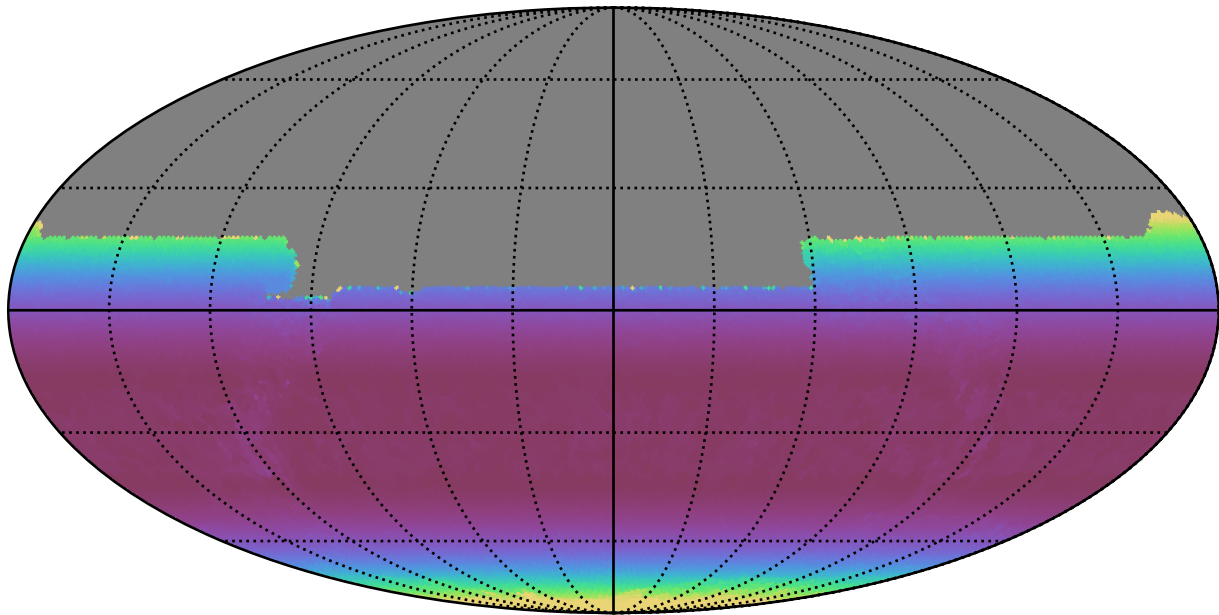
ddf_acor_sf25_lsf30_lsr50_v3.4_10yrs All sky y band: Min airmass
