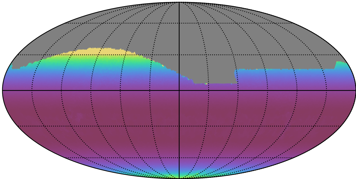
ddf_acor_sf25_lsf30_lsr50_v3.4_10yrs All sky r band: Min airmass
