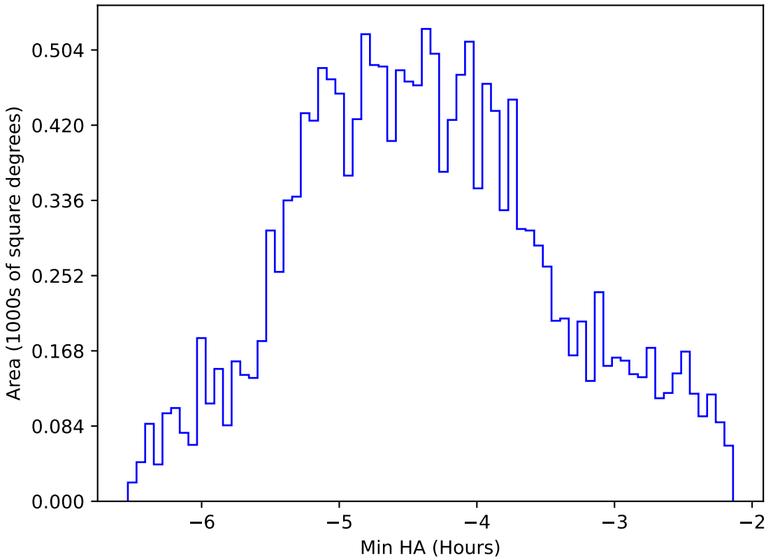
ddf_acor_sf25_lsf30_lsr50_v3.4_10yrs WFD z band: Min HA
