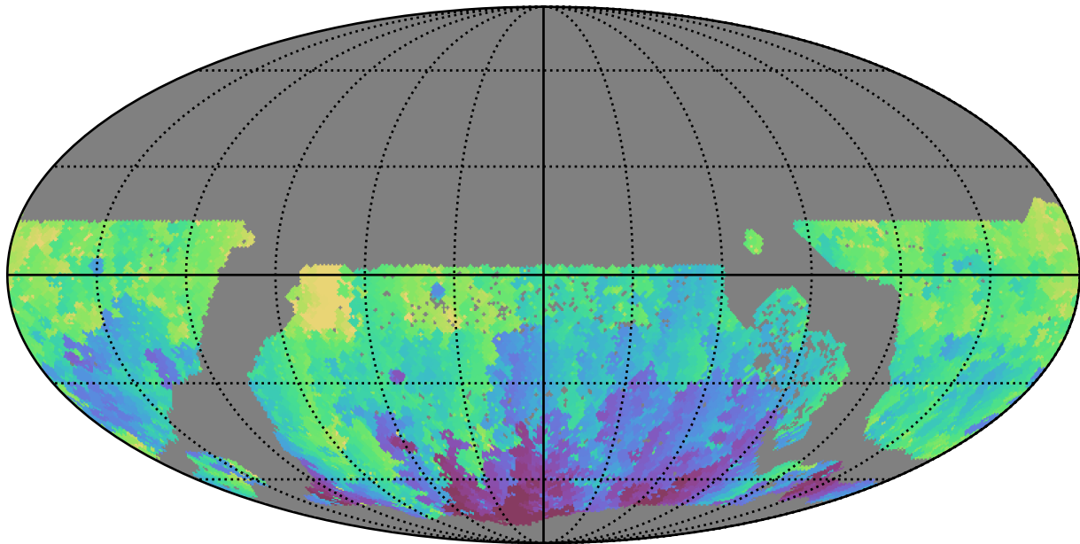
ddf_acor_sf25_lsf30_lsr50_v3.4_10yrs WFD u band: Min HA
