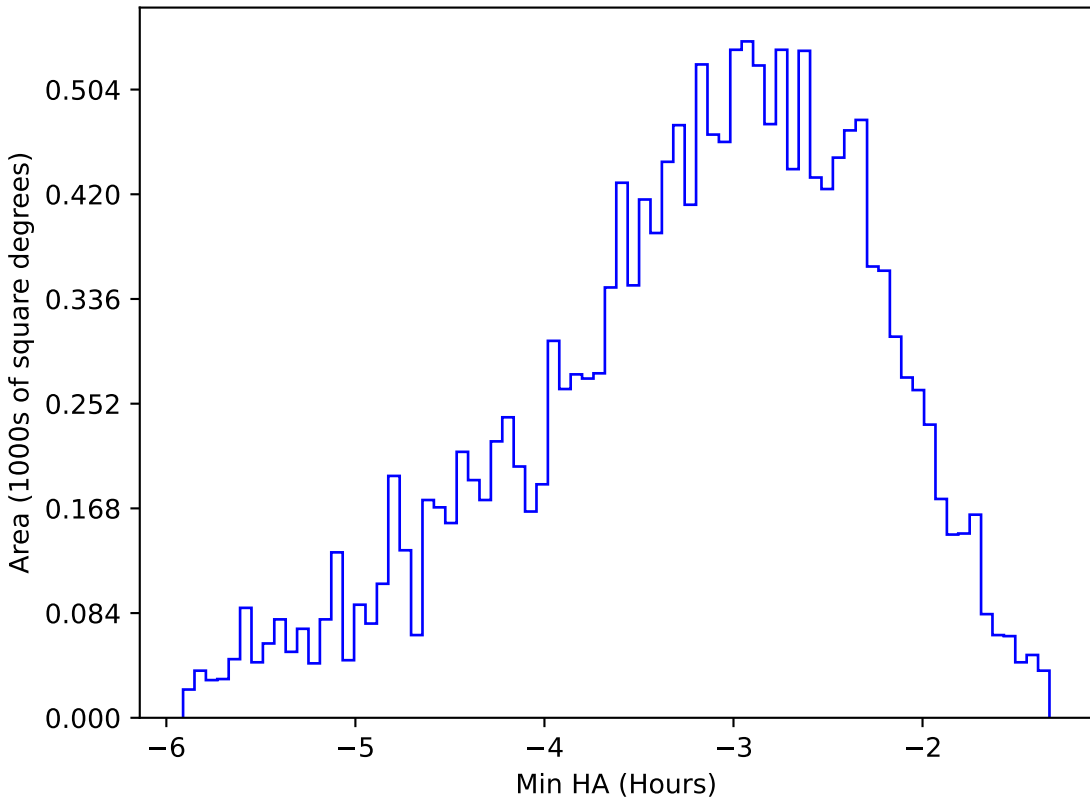
ddf_acor_sf25_lsf30_lsr50_v3.4_10yrs WFD u band: Min HA
