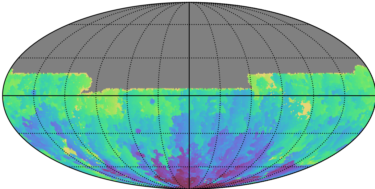
ddf_acor_sf25_lsf30_lsr50_v3.4_10yrs All sky u band: Min HA
