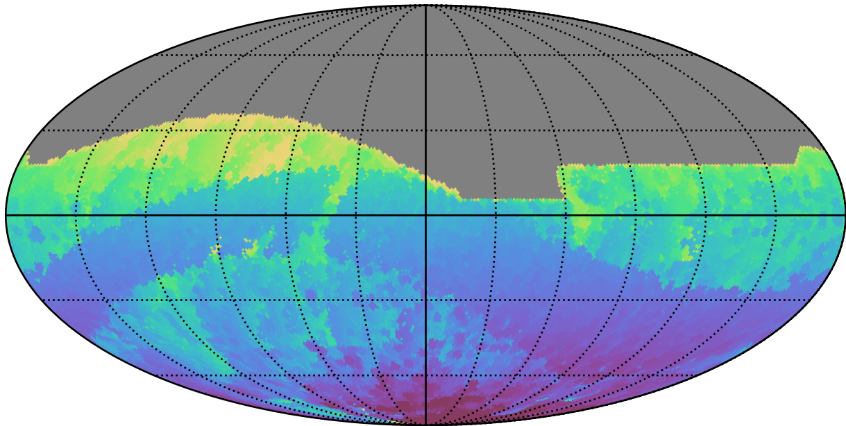
ddf_acor_sf25_lsf30_lsr50_v3.4_10yrs All sky r band: Min HA
