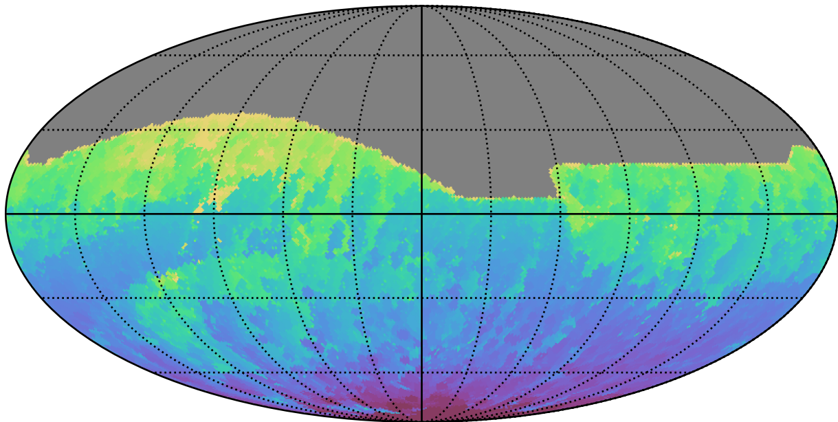
ddf_acor_sf25_lsf30_lsr50_v3.4_10yrs All sky i band: Min HA
