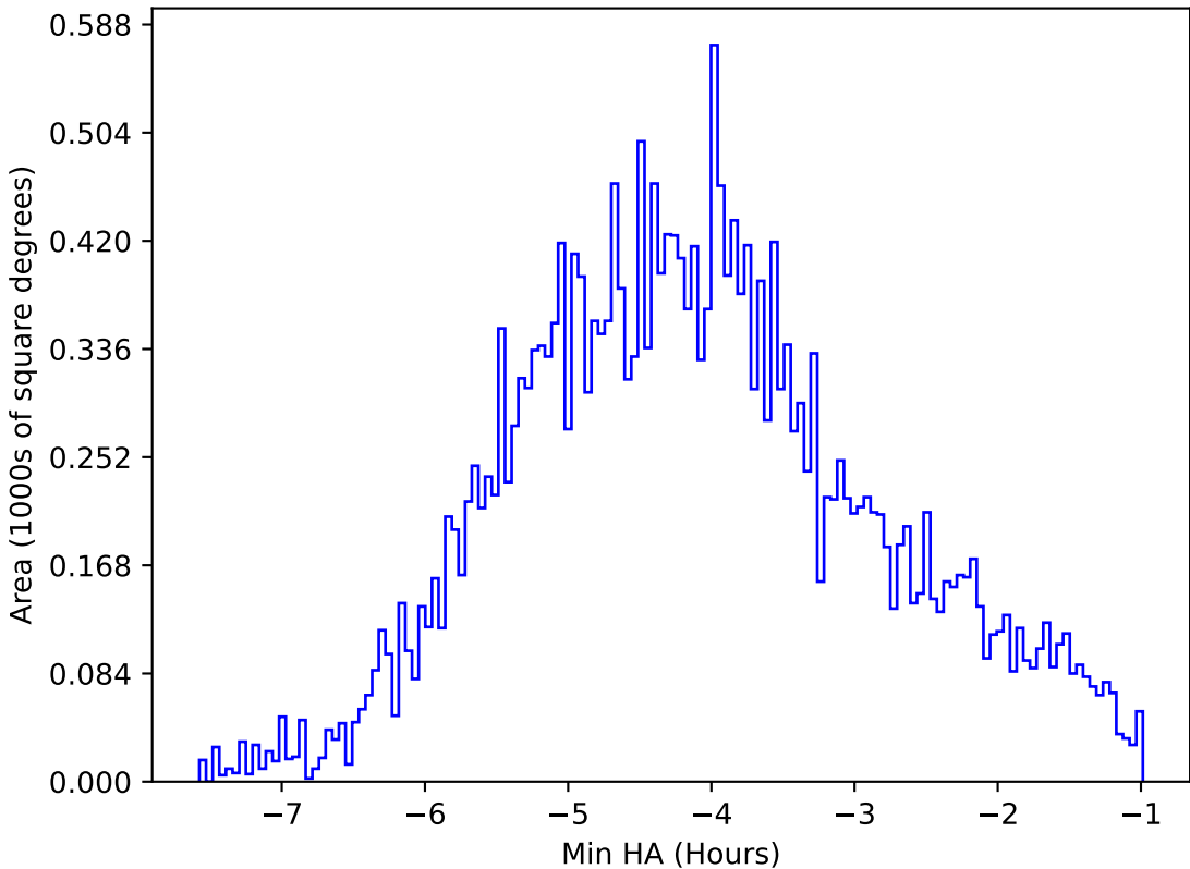
ddf_acor_sf25_ls30_lsr50_v3.4_10yrs All sky i band: Min HA
