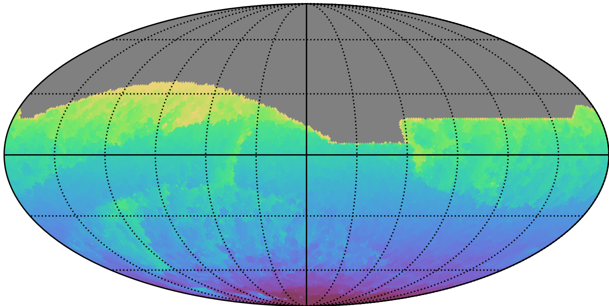
ddf_acor_sf25_lsf30_lsr50_v3.4_10yrs All sky all bands: Min HA
