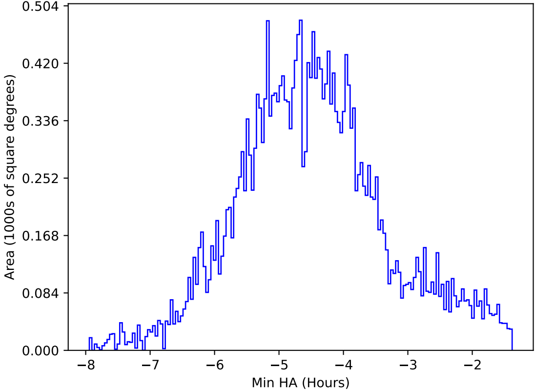
ddf_acor_sf25_lsf30_lsr50_v3.4_10yrs All sky all bands: Min HA
