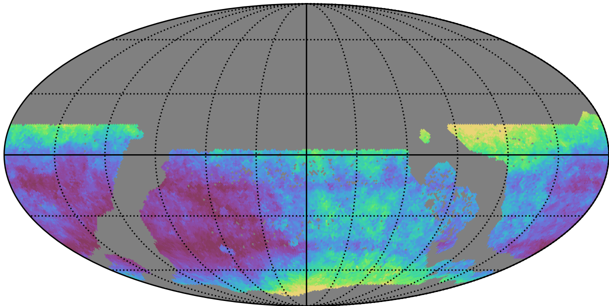
ddf_acor_sf25_lsf30_lsr50_v3.4_10yrs WFD i band: Median seeingEff
