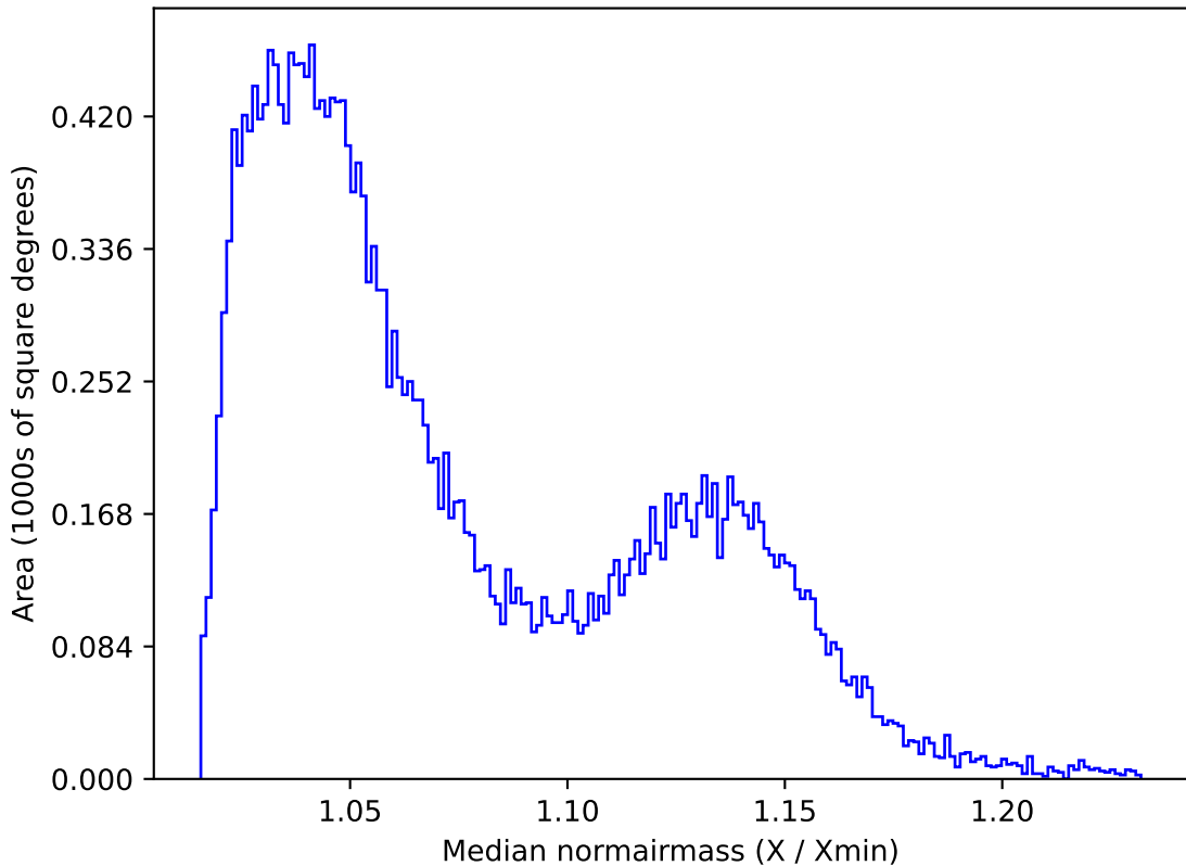
ddf_acor_sf25_lsf30_lsr50_v3.4_10yrs All sky i band: Median normairmass
