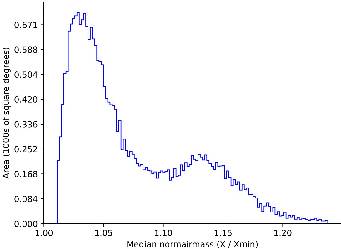
ddf_acor_sf25_lsf30_lsr50_v3.4_10yrs All sky g band: Median normairmass
