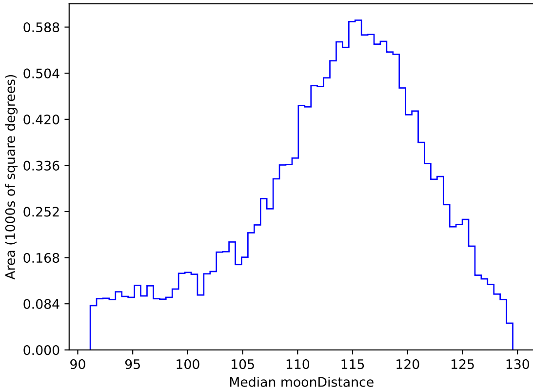
ddf_acor_sf25_lsf30_lsr50_v3.4_10yrs WFD r band: Median moonDistance
