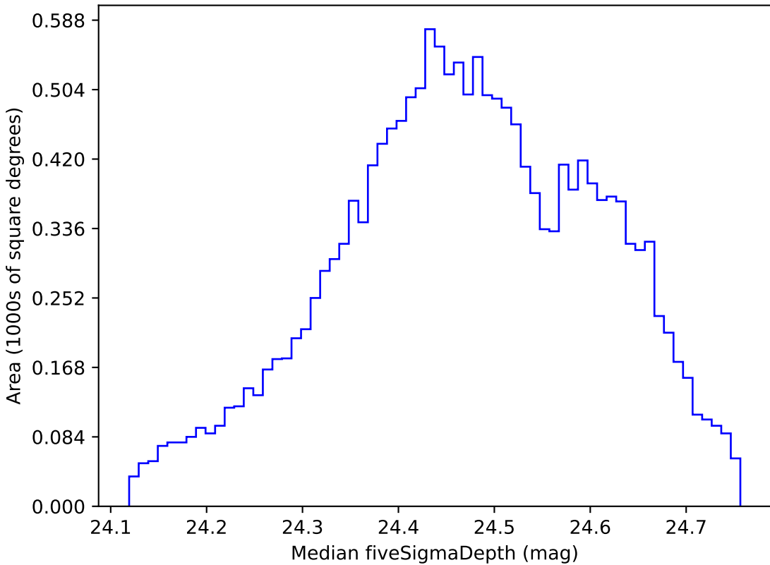
ddf_acor_sf25_lsf30_lsr50_v3.4_10yrs WFD g band: Median fiveSigmaDepth
