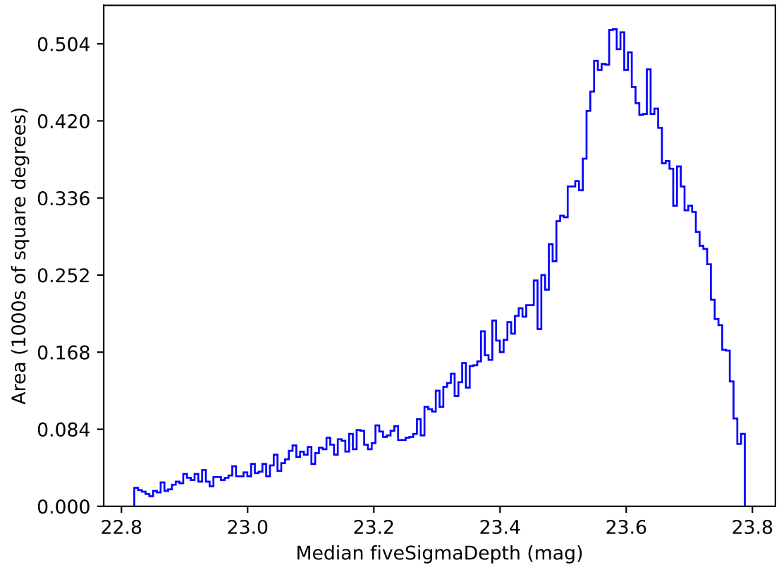
ddf_acor_sf25_lsf30_lsr50_v3.4_10yrs All sky i band: Median fiveSigmaDepth
