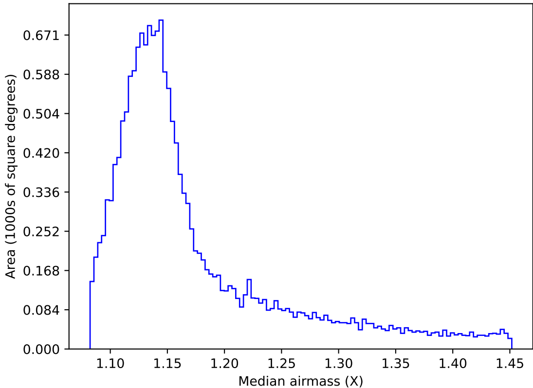
ddf_acor_sf25_lsf30_lsr50_v3.4_10yrs WFD i band: Median airmass
