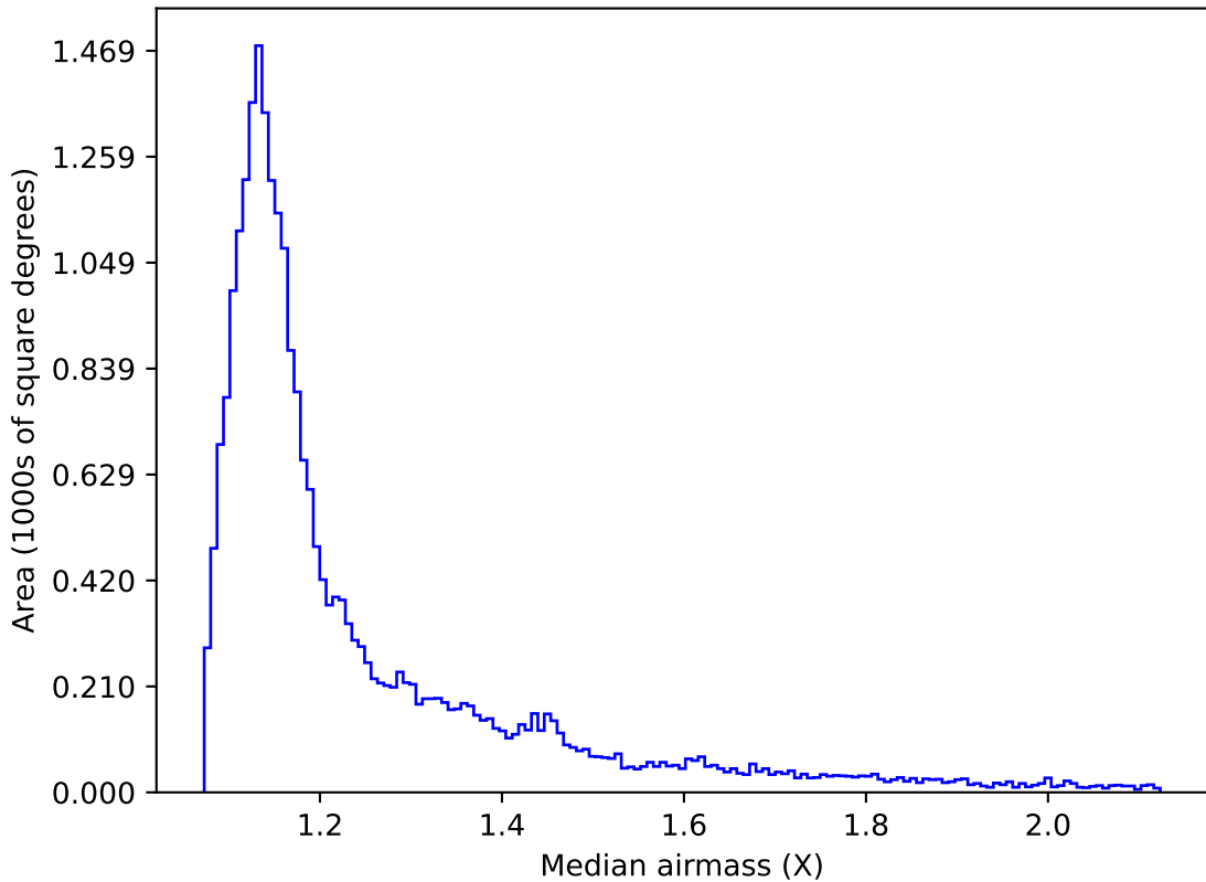
ddf_acor_sf25_lsf30_lsr50_v3.4_10yrs All sky g band: Median airmass
