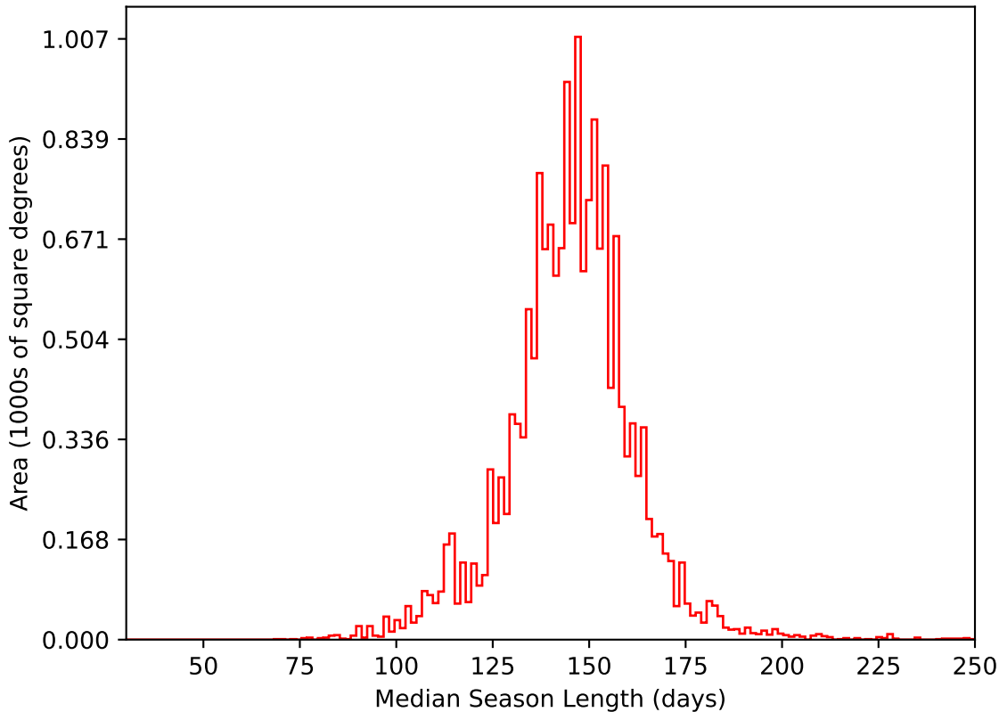
ddf_acor_sf25_lsf30_lsr50_v3.4_10yrs WFD i band: Median Season Length
