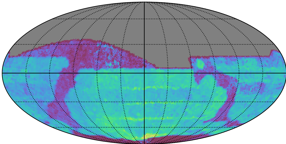
ddf_acor_sf25_lsf30_lsr50_v3.4_10yrs All sky z band: Median Season Length
